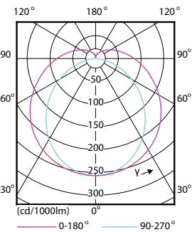
Light Distribution Diagram - MAS LEDtube 1200mm HO 14W830 T8
