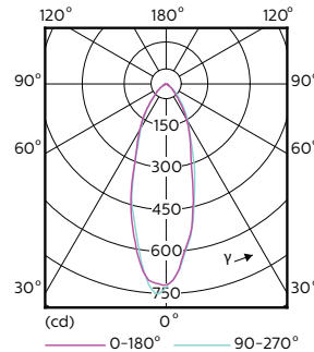
Light Distribution Diagram - 4.5GU10/LEDCLA/F35/830/DIM 10/1
