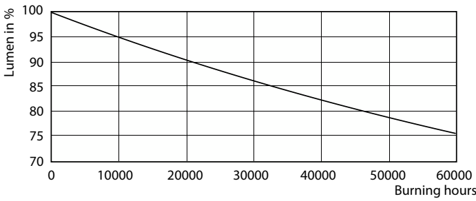
Lumen Maintenance Diagram - MAS MR16 ExpertColor7.2-50W 927 10D EZ10
