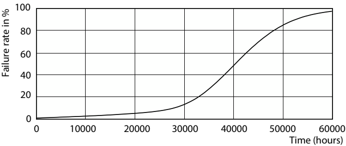
Life Expectancy Diagram - MAS MR16 ExpertColor7.2-50W 927 10D EZ10
