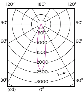
Light Distribution Diagram - MAS MR16 ExpertColor7.2-50W 930 24D EZ10
