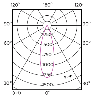
Light Distribution Diagram - MAS MR16 ExpertColor7.2-50W 927 36D EZ10
