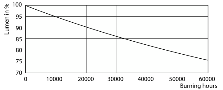
Lumen Maintenance Diagram - MAS MR16 ExpertColor7.2-50W 927 36D EZ10
