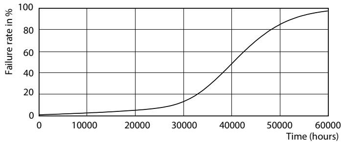
Life Expectancy Diagram - MAS MR16 ExpertColor7.2-50W 927 36D EZ10
