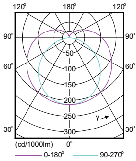
Light Distribution Diagram - 14T8/48-3500 IF 10/1 ROT
