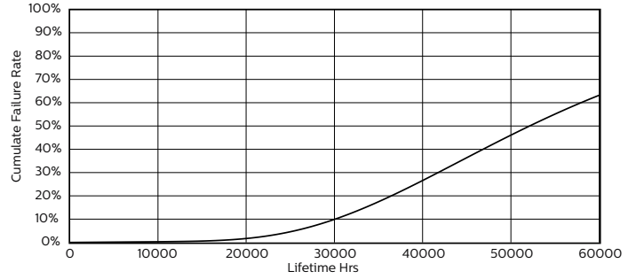
Life Expectancy Diagram - 14T8/48-3500 IF 10/1 ROT
