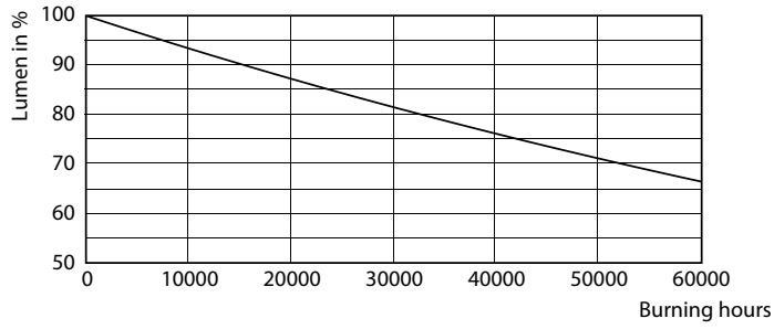
Lumen Maintenance Diagram - 14T8/48-3500 IF 10/1 ROT
