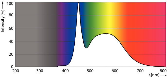
Spectral Power Distribution Colour - LEDBulb 8-70W E27 865 220-240V 1PF/10
