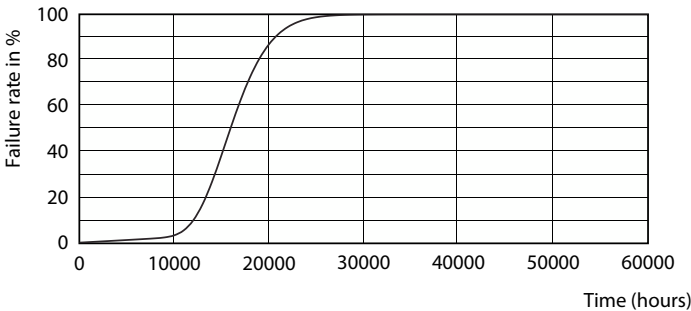
Life Expectancy Diagram - LEDBulb 8-70W E27 865 220-240V 1PF/10
