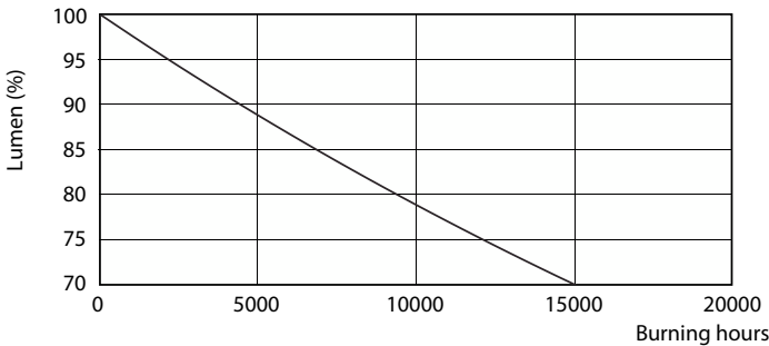
Lumen Maintenance Diagram - LEDBulb 8-70W E27 865 220-240V 1PF/10
