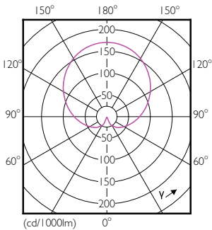
Light Distribution Diagram - LEDBulb 8-70W E27 865 220-240V 1PF/10
