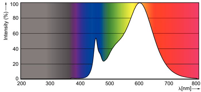
General Uniform Lighting TLED Ess IF 4000lm 3000K 8ft single pin Page 10
