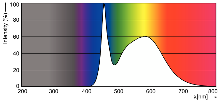
Spectral Power Distribution Colour - 7T8 LED/24-5000 IF 10/1
