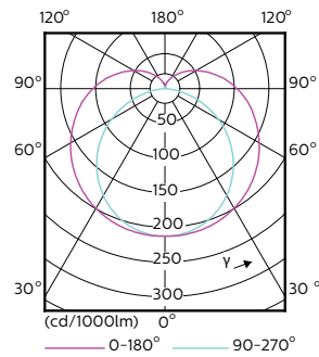
Light Distribution Diagram - 7T8 LED/24-5000 IF 10/1
