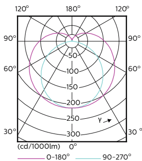
Light Distribution Diagram - 9T8 LED/36-5000 IF 10/1
