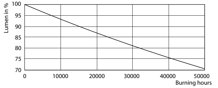
Lumen Maintenance Diagram - 9T8 LED/36-5000 IF 10/1
