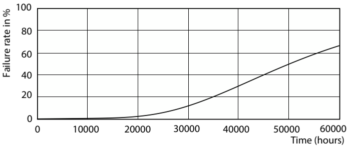
Life Expectancy Diagram - 13T8 LED/24-3000 IF-6U 10/1
