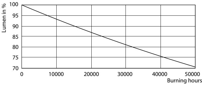
Lumen Maintenance Diagram - 13T8 LED/24-3000 IF-6U 10/1
