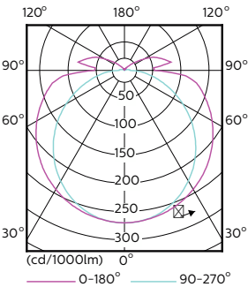
Light Distribution Diagram - 13T8 LED/24-3000 IF-6U 10/1
