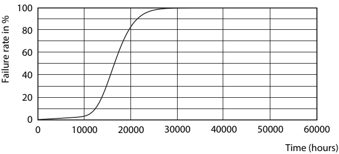
Life Expectancy Diagram - ESS LEDBulb 14W E27 6500K HV 1PF/20 AR
