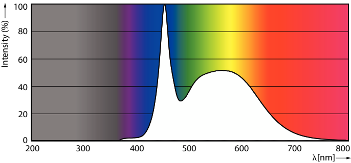
Spectral Power Distribution Colour - ESS LEDBulb 14W E27 6500K HV 1PF/20 AR
