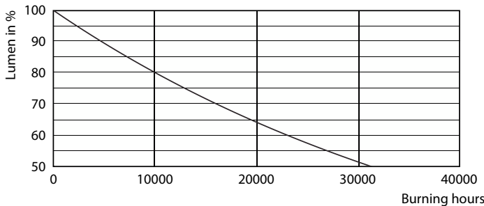
Lumen Maintenance Diagram - CorePro LEDbulb ND 18-120W E27 840 A67
