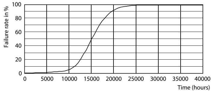
Life Expectancy Diagram - 6G25/AMB/822-27/E26/CL/GL/WGD BC 2PK
