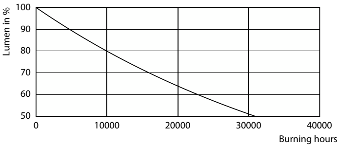
Lumen Maintenance Diagram - 6G25/AMB/822-27/E26/CL/GL/WGD BC 2PK
