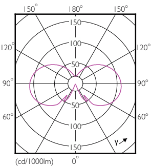
Light Distribution Diagram - 6G25/AMB/822-27/E26/CL/GL/WGD BC 2PK
