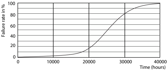
Life Expectancy Diagram - 7PAR20/LED/F25/830/E26/GL/DIM 120V
