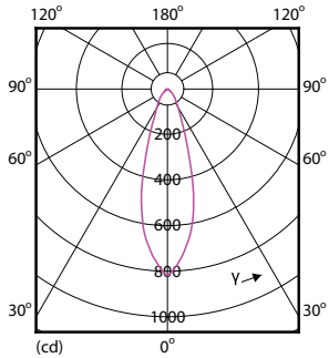
LEDspot PAR20 7W 830 500lm 25D
