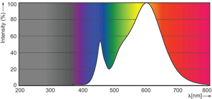
Spectral Power Distribution Colour - 7PAR20/LED/F40/830/E26/GL/DIM 120V
