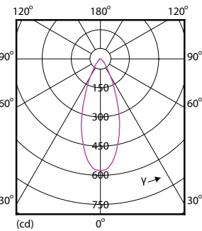
Light Distribution Diagram - 7PAR20/LED/F40/830/E26/GL/DIM 120V
