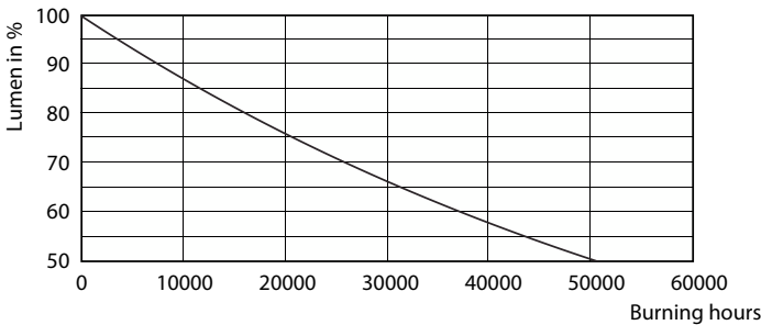
Lumen Maintenance Diagram - 7PAR20/LED/F40/830/E26/GL/DIM 120V
