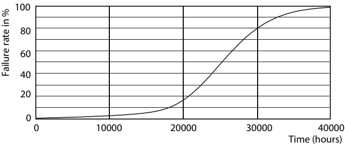
Life Expectancy Diagram - 7PAR20/LED/F40/830/E26/GL/DIM 120V
