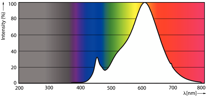
Spectral Power Distribution Colour - MAS LEDspot D 6-50W E27 827 PAR20 25D
