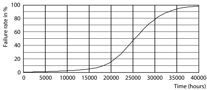
Life Expectancy Diagram - 5.5PAR16/AMB/F40/830/E26/DIM120V BC 1PK
