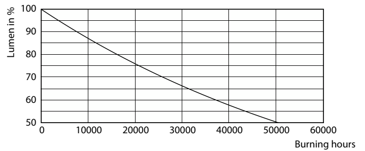
Lumen Maintenance Diagram - 5.5PAR16/AMB/F40/830/E26/DIM120V BC 1PK
