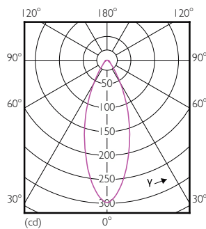
Light Distribution Diagram - 5.5PAR16/AMB/F40/830/E26/DIM120V BC 1PK
