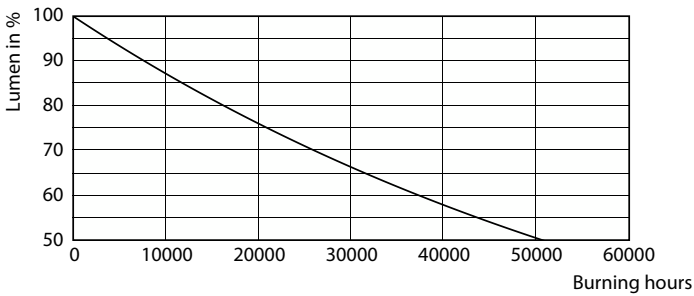
Lumen Maintenance Diagram - 12PAR38/LED/827/F25/DIM/ULW/120V 6/1FB
