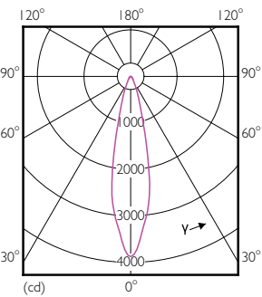
Light Distribution Diagram - 12PAR38/LED/827/F25/DIM/ULW/120V 6/1FB
