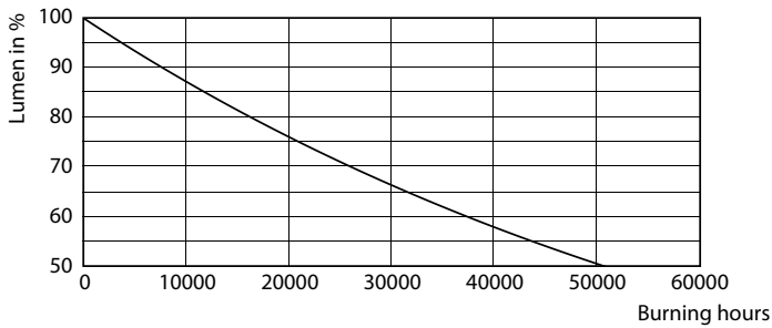
Lumen Maintenance Diagram - 12PAR38/LED/830/F25/DIM/ULW/120V 6/1FB
