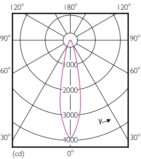
Light Distribution Diagram - 12PAR38/LED/830/F25/DIM/ULW/120V 6/1FB
