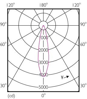
Light Distribution Diagram - 12PAR38/LED/840/F25/DIM/ULW/120V 6/1FB
