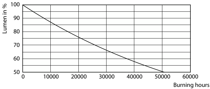
Lumen Maintenance Diagram - 12PAR38/LED/840/F25/DIM/ULW/120V 6/1FB
