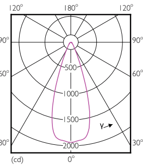
Light Distribution Diagram - 12PAR38/LED/827/F40/DIM/ULW/120V 6/1FB
