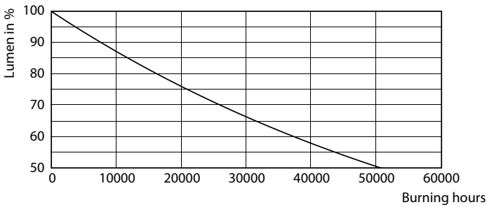
Lumen Maintenance Diagram - 12PAR38/LED/830/F40/DIM/ULW/120V 6/1FB
