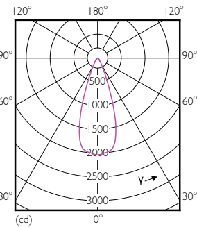
Light Distribution Diagram - 12PAR38/LED/830/F40/DIM/ULW/120V 6/1FB
