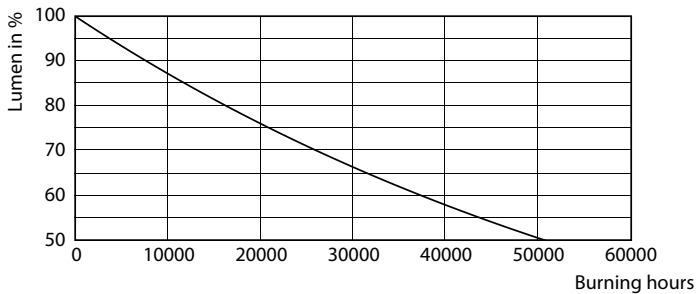
Lumen Maintenance Diagram - 10PAR30S/LED/827/F25/DIM/ULW/120V 6/1FB
