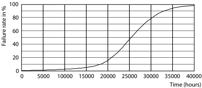
Life Expectancy Diagram - 10PAR30S/LED/830/F25/DIM/ULW/120V 6/1FB
