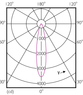
Light Distribution Diagram - 10PAR30S/LED/830/F25/DIM/ULW/120V 6/1FB
