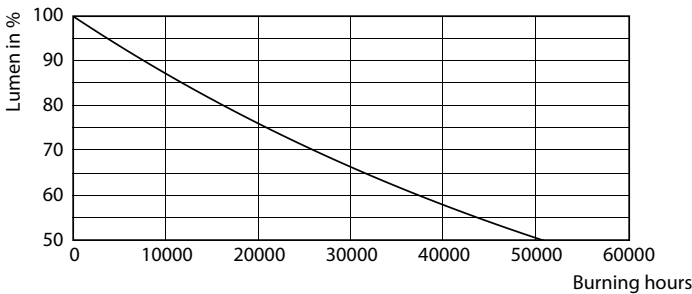
Lumen Maintenance Diagram - 10PAR30S/LED/830/F25/DIM/ULW/120V 6/1FB
