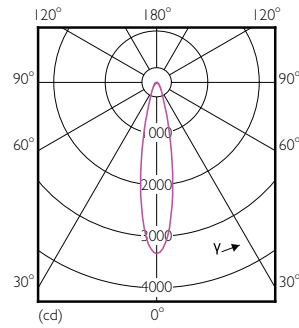
Light Distribution Diagram - 10PAR30L/LED/827/F25/DIM/ULW/120V 6/1FB
