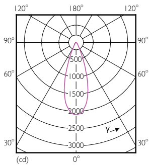
Light Distribution Diagram - 10PAR30L/AMB/830/F40/GL/D ULW BC 1PK 4/1
