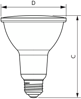
10PAR30L/LED/830/F40/DIM/ULW/120V 6/1FB
