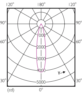
Light Distribution Diagram - MAS LEDspot CLA D 9.5-75W 840 PAR30S 25D
