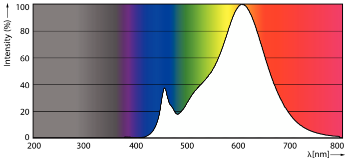
Spectral Power Distribution Colour - CorePro LEDcapsule ND 1.9-25W G9 827
