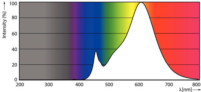
Spectral Power Distribution Colour - CorePro LEDcapsule ND 1.9-25W G9 827
