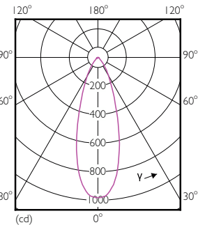
Light Distribution Diagram - MAS LED spot VLE D 5.5-35W MR16 827 36D
