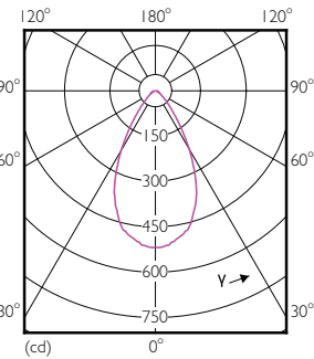
Light Distribution Diagram - MAS LED spot VLE D 5.5-35W MR16 840 60D
