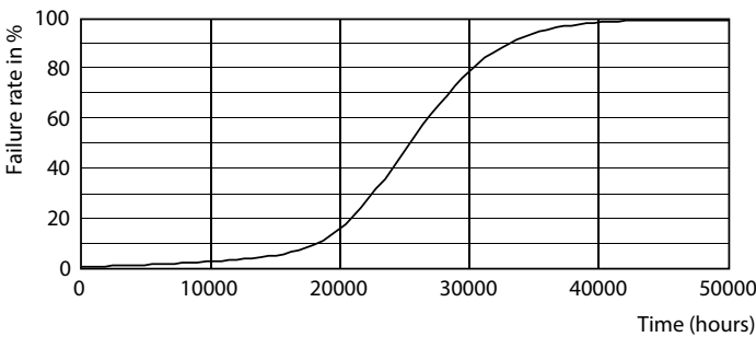
Life Expectancy Diagram - MAS LED spot VLE D 5.5-35W MR16 840 60D
