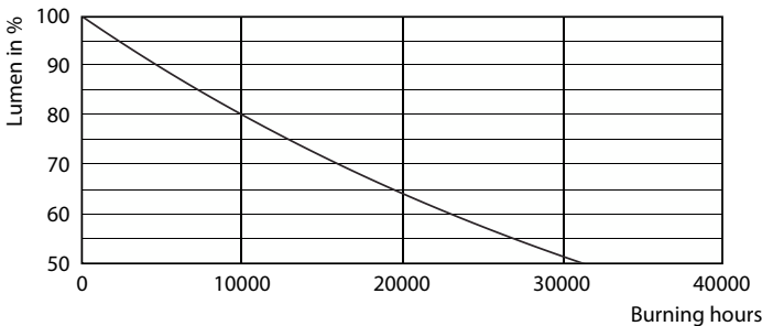
Lumen Maintenance Diagram - CLA LEDBulb D 5-40W A60 B22 827 CL
