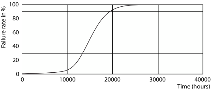
Life Expectancy Diagram - CLA LEDBulb D 5-40W A60 B22 827 CL
