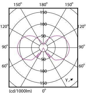
Light Distribution Diagram - CLA LEDBulb D 5-40W A60 B22 827 CL
