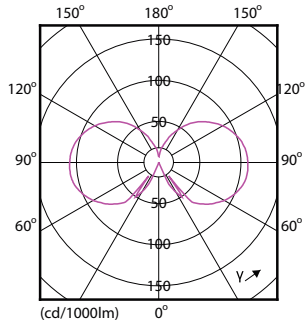
Light Distribution Diagram - CLA LEDLuster D 2.7-25W P45 E27 827 CL
