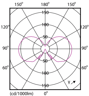
Light Distribution Diagram - CLA LEDBulb D 7.5-48W A60 B22 820 GOLD
