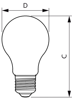
Bulb A60 4.5-40W470lm 2000-2700K D Clear
