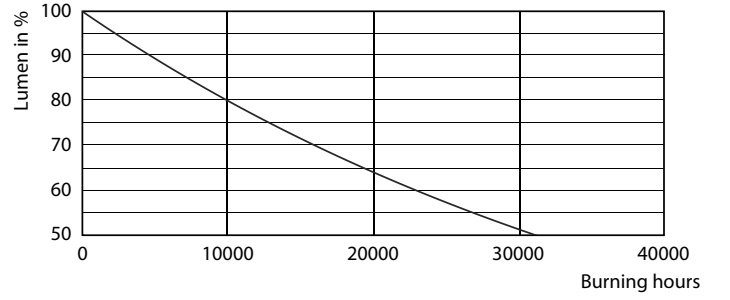
Lumen Maintenance Diagram - CLA LEDBulb DT 8-60W ST64 E27 CL
