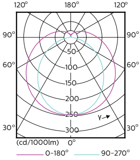
Light Distribution Diagram - MAS LEDtube UN 1500mm UO 24W840 T8
