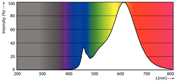
Spectral Power Distribution Colour - LED SSW 100W A67 E27 WW FR ND 1BC/6
