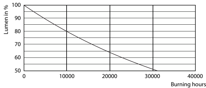
Lumen Maintenance Diagram - LED SSW 100W A67 E27 WW FR ND 1BC/6
