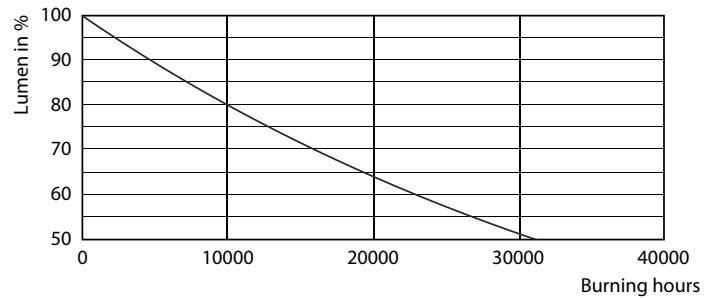
Lumen Maintenance Diagram - LED SSW 100W A67 E27 WW FR ND 1SRT4
