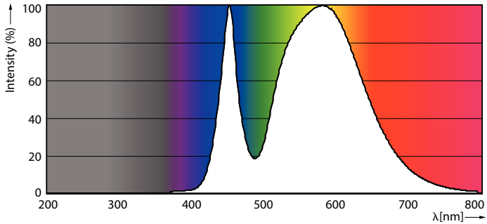
Spectral Power Distribution Colour - Ecofit LEDtube 1500mm 20W 840 T8
