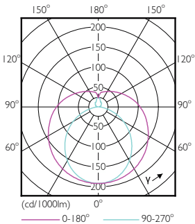
Light Distribution Diagram - Ecofit LEDtube 1500mm 20W 840 T8
