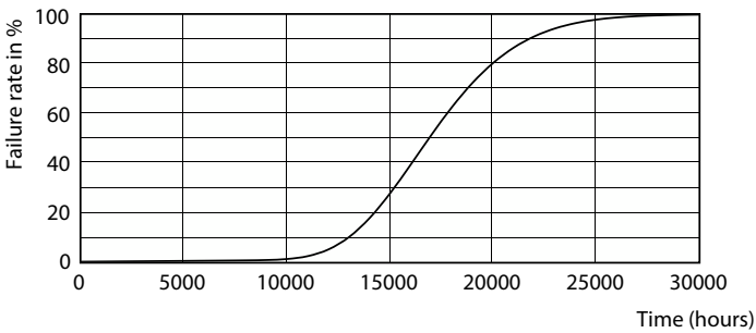
Life Expectancy Diagram - Ecofit LEDtube 1500mm 20W 840 T8
