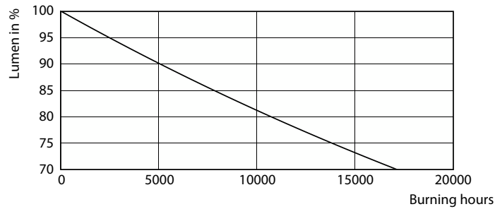
Lumen Maintenance Diagram - Ecofit LEDtube 1500mm 20W 840 T8
