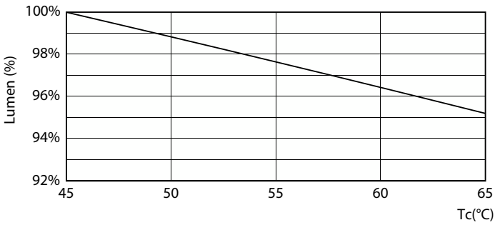
Lumen Maintenance Diagram - Ecofit LEDtube 1500mm 20W 840 T8
