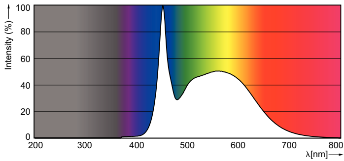
LEDtube 1200mm 15W G13 865 1600lm
