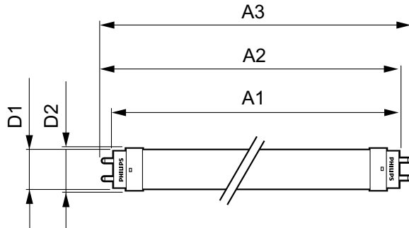
TLED 4ft 14.5-36W 1600lm 6500K G13 Ess
