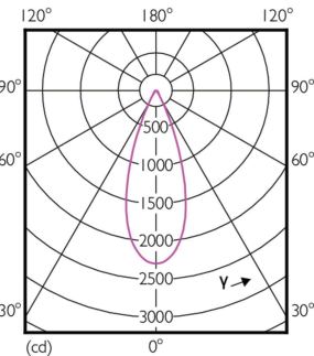
Light Distribution Diagram - 12PAR30S/EXPERTCOLOR/F40/940/DIM
