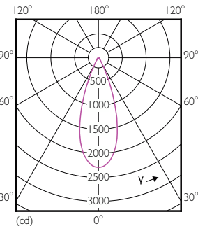
Light Distribution Diagram - 12PAR30L/EXPERTCOLOR/F40/940/DIM
