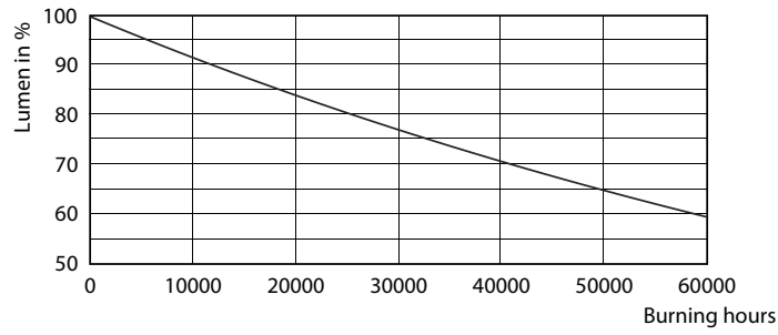
Lumen Maintenance Diagram - 12PAR30L/EXPERTCOLOR/F40/940/DIM
