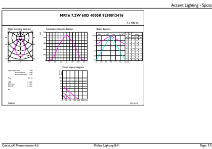
Accent Lighting Spots - MAS LED MR16 ExpertColor 7.2-50W 940 60D
