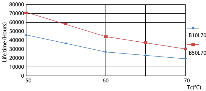
Life Expectancy Diagram - 14T8 PRO LED/48-4000 IF G 10/1
