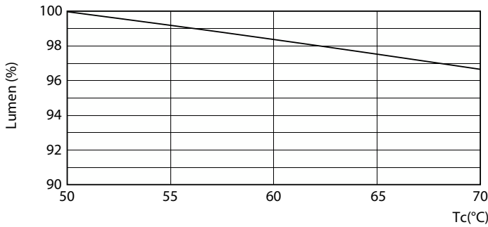
Lumen Maintenance Diagram - 14T8 PRO LED/48-4000 IF G 10/1
