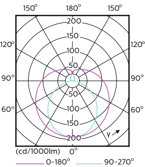
Light Distribution Diagram - 14T8 PRO LED/48-4000 IF G 10/1
