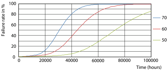
Life Expectancy Diagram - 14T8 PRO LED/48-4000 IF G 10/1
