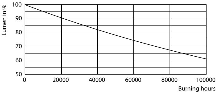
Lumen Maintenance Diagram - 14T8 PRO LED/48-4000 IF G 10/1
