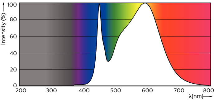
Spectral Power Distribution Colour - 14T8 PRO LED/48-4000 IF G 10/1
