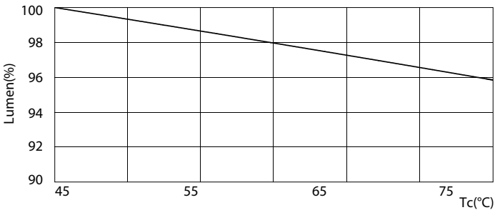
Lumen Maintenance Diagram - 17T8 LED/48-4000 IF G 10/1
