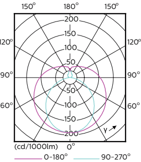
Light Distribution Diagram - 17T8 LED/48-4000 IF G 10/1
